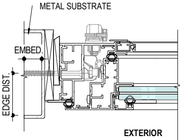
4 106 ANCHORAGE INTO METAL STRUCTURE NOT TO SCALE
