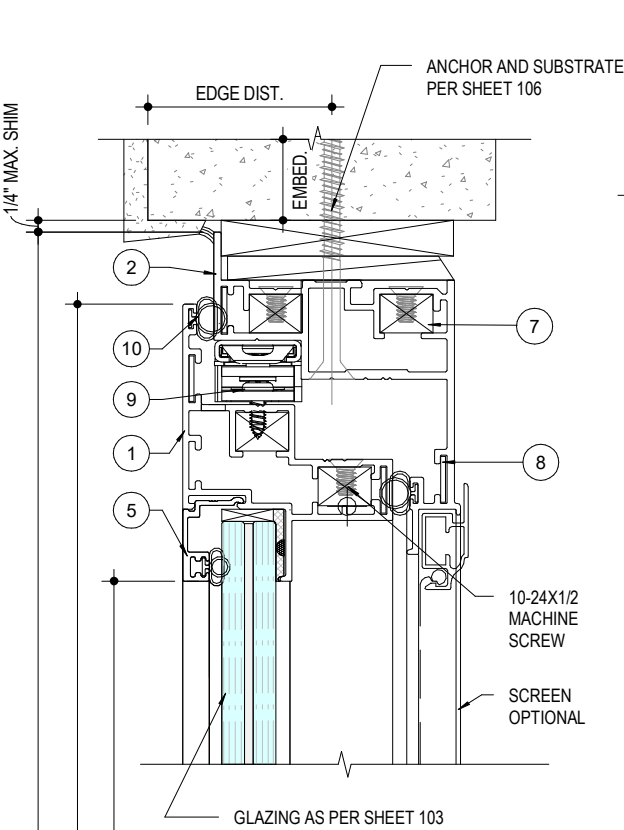
2 104 CASEMENT LOCK JAMB DETAIL NOT TO SCALE
