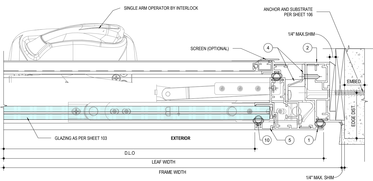
3 104 CASEMENT JAMB DETAIL NOT TO SCALE
