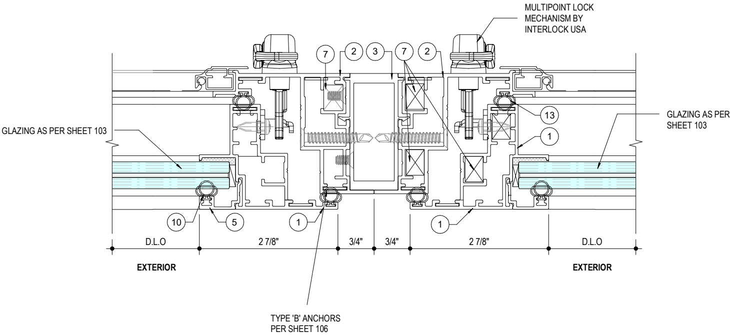
4 104 CASEMENT INTERMEDIATE MULLION DETAIL NOT TO SCALE
