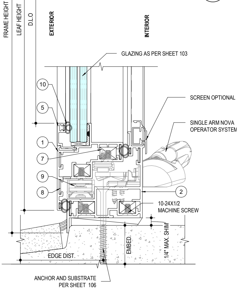
1 104 CASEMENT SILL AND HEAD DETAIL NOT TO SCALE
