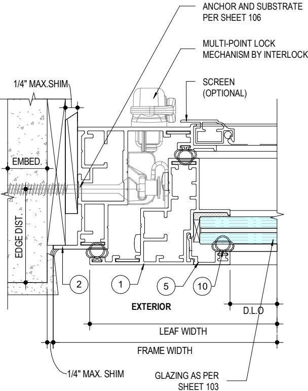
2 104 CASEMENT LOCK JAMB DETAIL NOT TO SCALE
