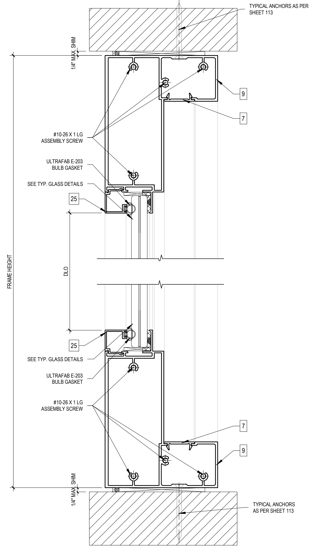
2 108 SIDELITE HEAD/SILL DETAIL 6" = 1'-0"
