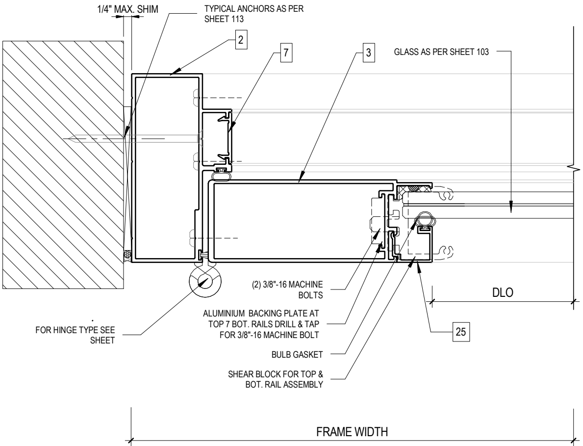
3 109 DOOR HINGED JAMB DETAIL 1 6" = 1'-0"
