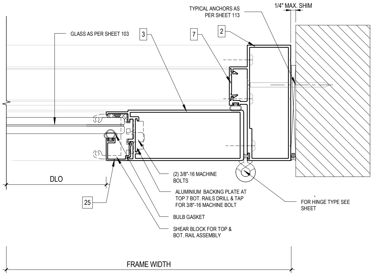
4 109 DOOR HINGED JAMB DETAIL 2 6" = 1'-0"
