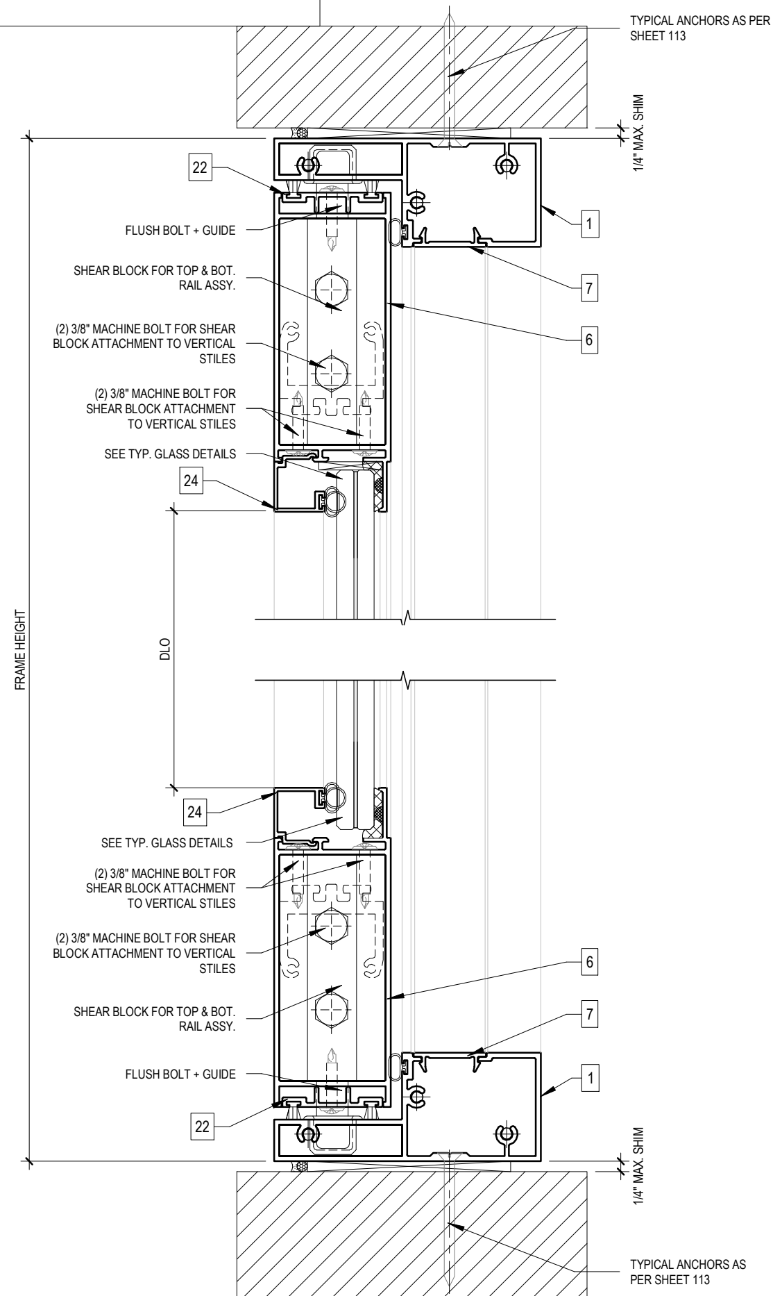
DOOR HEAD/SILL 6" = 1'-0"
