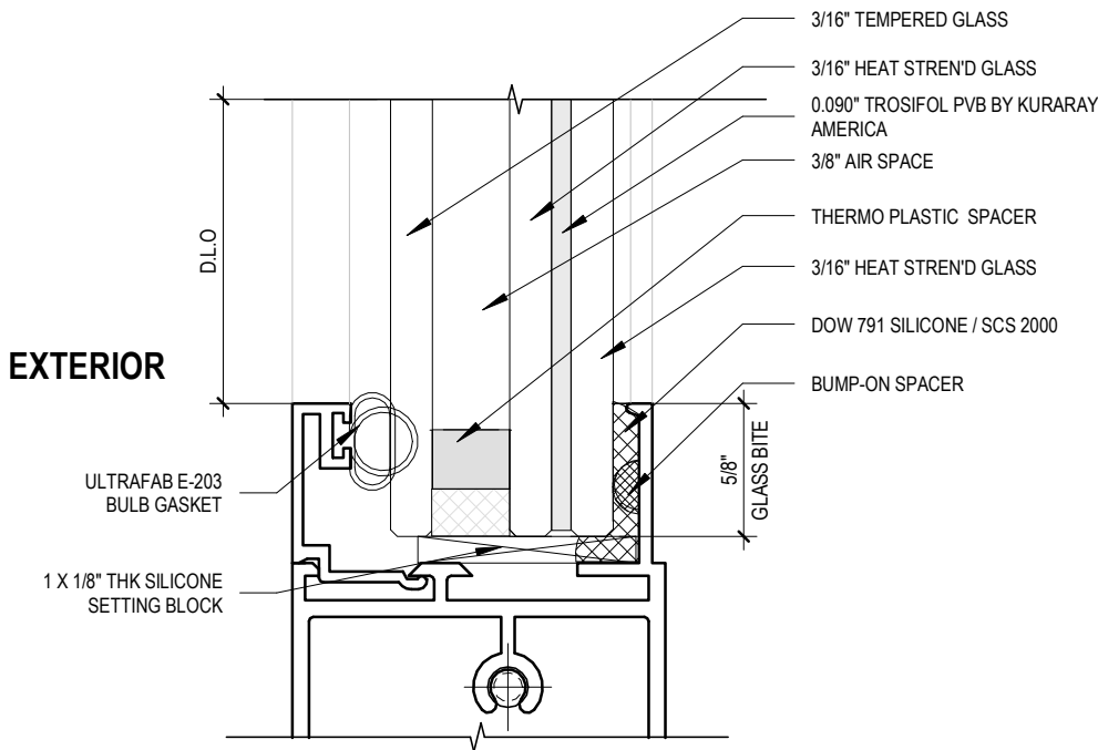
1 103 GLAZING DETAIL (GL-1) 12" = 1'-0"
