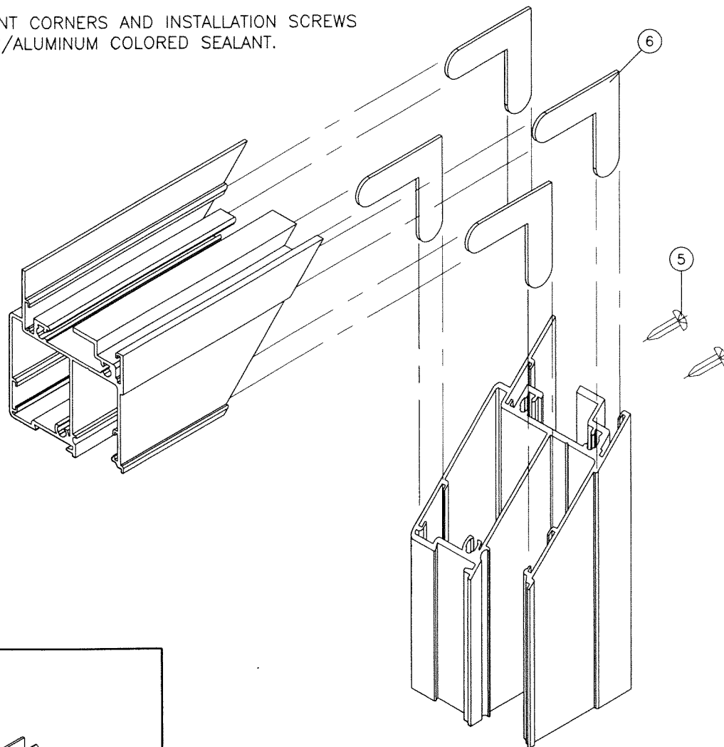
FRAME CORNER
