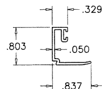
3A GLAZING STOP (LAM. GLASS)
