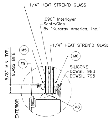
GLASS TYPE 'B' 9/16" OVERALL LAM. GLASS
