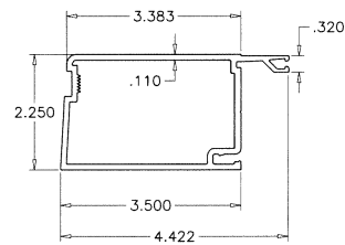
E6 HINGE/LOCK STILE
