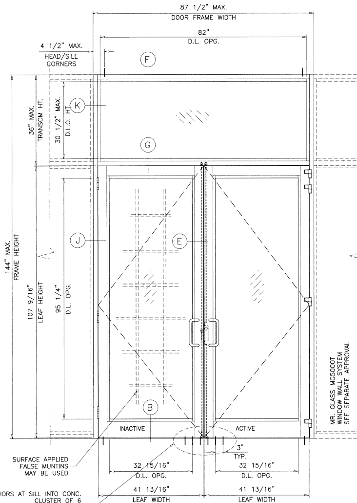
TYPICAL ELEVATION DOUBLE (O/XX) (ES-8000T TRANSOM)
