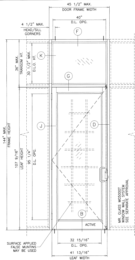
TYPICAL ELEVATION SINGLE (O/X) (ES-8000T TRANSOM)
