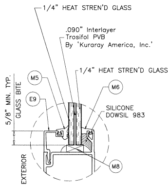
GLASS TYPE 'A.1' 9/16" OVERALL LAM. GLASS
