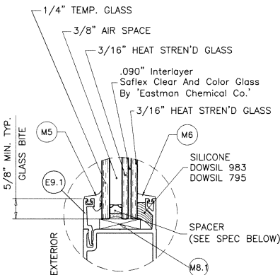
GLASS TYPE 'C.1' 1-1/8" OVERALL INSUL. LAM. GLASS
