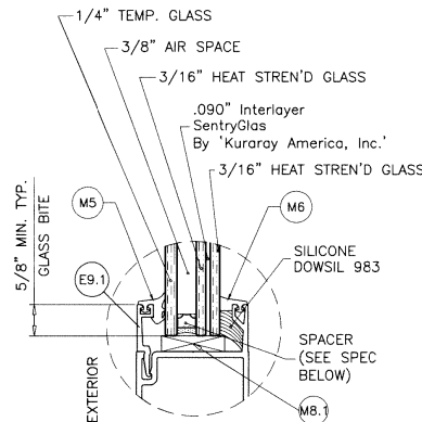
GLASS TYPE 'D' 1-1/8" OVERALL INSUL. LAM. GLASS
