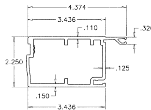
E8 MEETING STILE - INACTIVE LEAF
