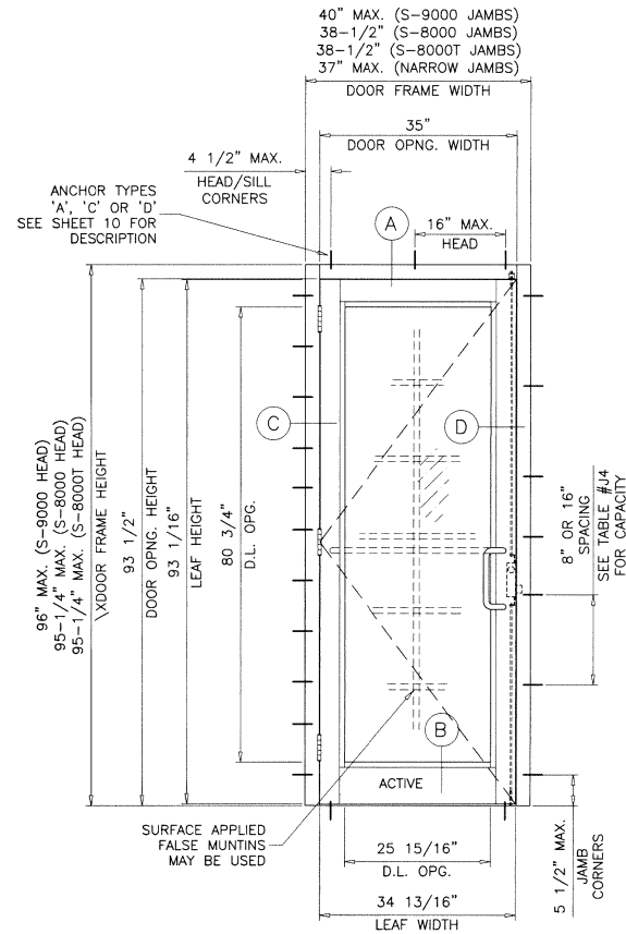
TYPICAL ELEVATION (X)
