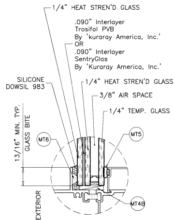
GLASS TYPE 'E'
