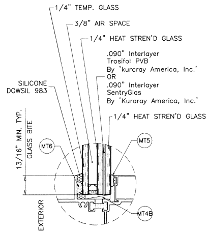
GLASS TYPE 'E-R'
