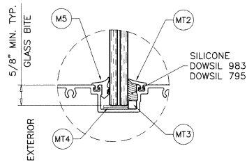
GLAZING DETAIL S-9500 TRANSOM
