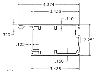
E7 MEETING STILE - ACTIVE LEAF
