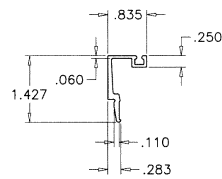
E9 GLASS STOP (LAM. GLASS)
