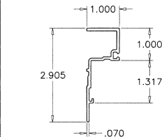
T2 TRANSOM ADAPTER
