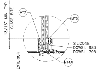
GLAZING DETAIL S-8000 TRANSOM
