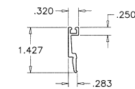
E9.1 GLASS STOP (INSUL. LAM. GLASS)
