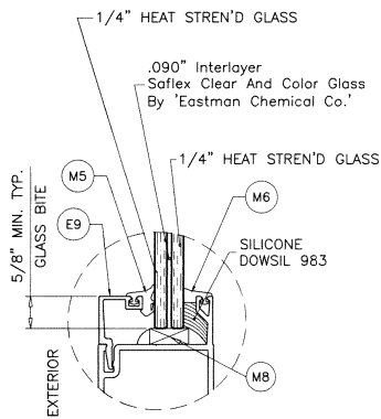
GLASS TYPE 'A.2' 9/16" OVERALL LAM. GLASS
