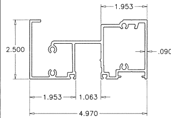
T1 TRANSOM HEADER Series 9500
