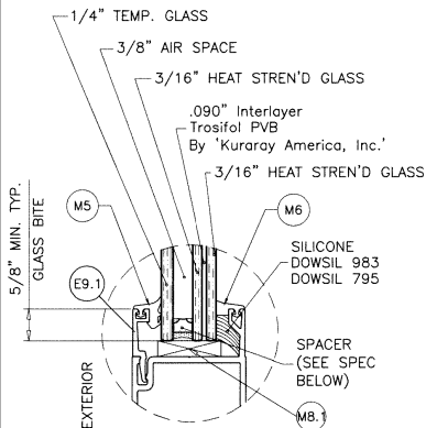
GLASS TYPE 'C' 1-1/8" OVERALL INSUL. LAM. GLASS
