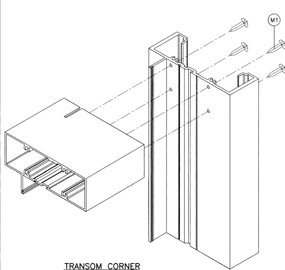
TRANSOM CORNER SERIES-MG5000 WINDOW WALL
