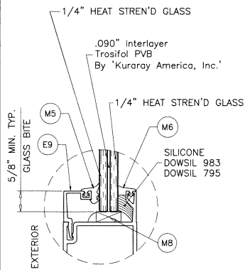
GLASS TYPE 'A' 9/16" OVERALL LAM. GLASS
