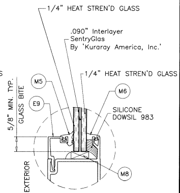
GLASS TYPE 'B.1' 9/16" OVERALL LAM. GLASS
