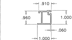
T3 TRANSOM GLASS STOP
