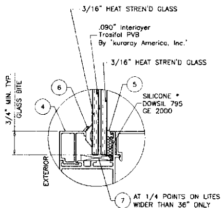
GLASS TYPE 'A' 7/16" OVERALL LAM. GLASS
