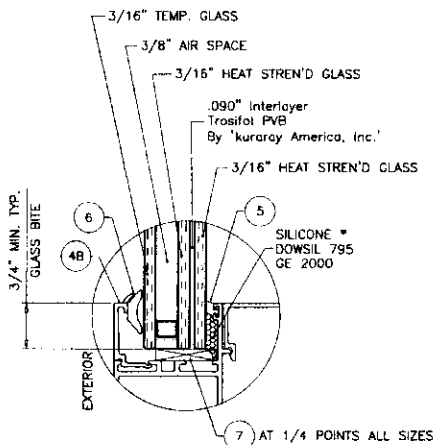
GLASS TYPE 'Ai' 13/16" OVERALL INSUL. LAM. GLASS
