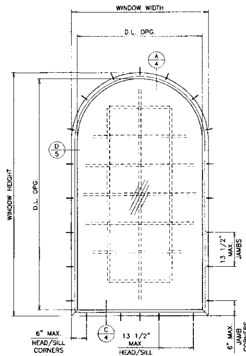
TYPICAL ELEVATIONS (TESTED UNITS)
